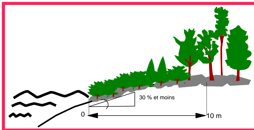
Figure 13.1b : Rive de 10 m (cas no 2)
