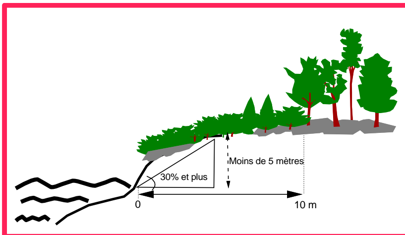
Figure 13.1b : Rive de 10 m (cas no 2)
