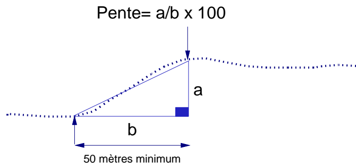
Figure 2.8c :Pente
